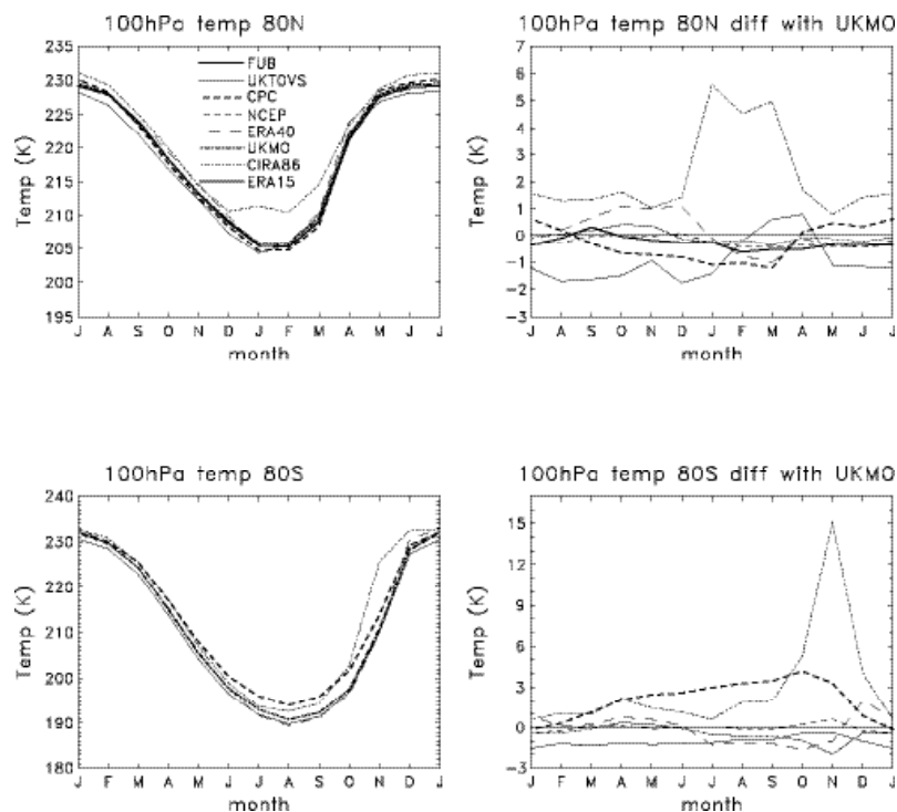
Figure 9. Left panels show seasonal variation of 100 hPa zonal mean temperature at 80°N (top) and 80°S (bottom); note the respective time axes have been shifted by 6 months so that winter is in the middle of each plot. Right panels show the respective differences from UKMO analyses.
