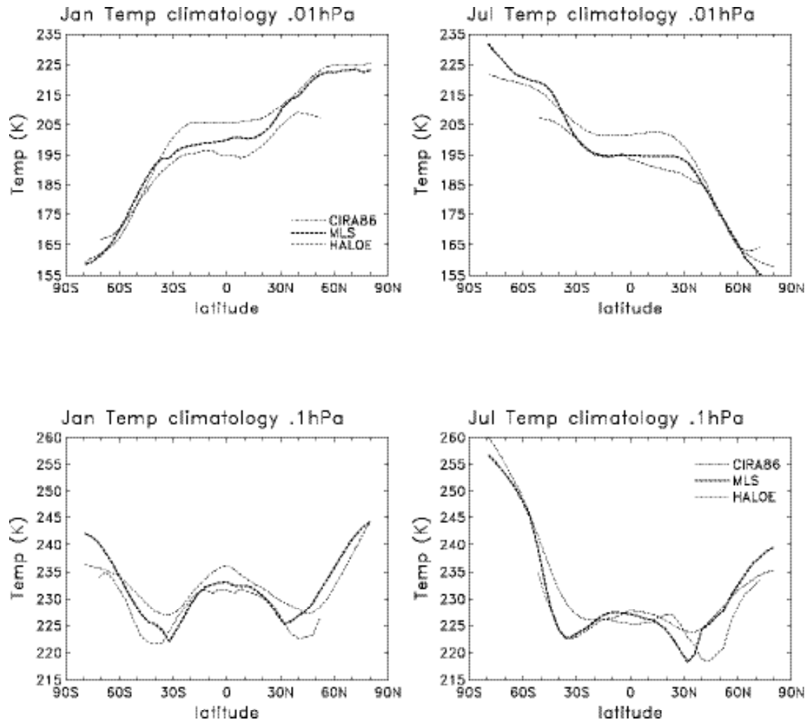
Figure 7. Latitudinal distribution of zonal mean temperatures at 0.01 hPa ( \sim 80 km) (top) and 0.1 hPa ( \sim 65 km) (bottom), for January (left) and July (right).
