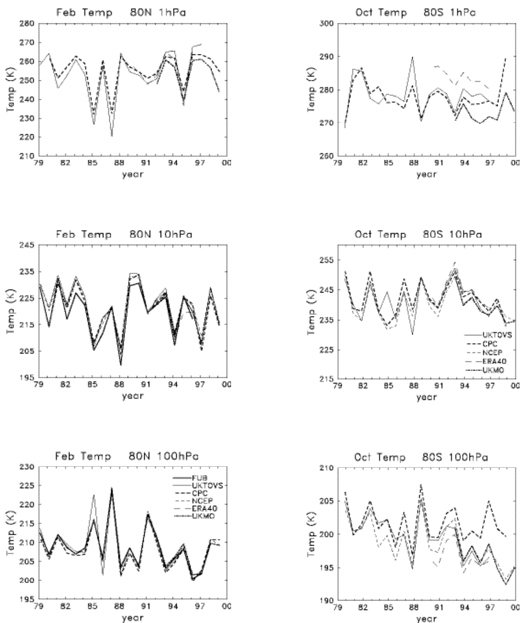
Figure 21. Time series of February average zonal mean temperatures at 80°N from each available data set, comparing interannual variability statistics. Results are shown for 1 hPa (top), 10 hPa (middle) and 100 hPa (bottom).
