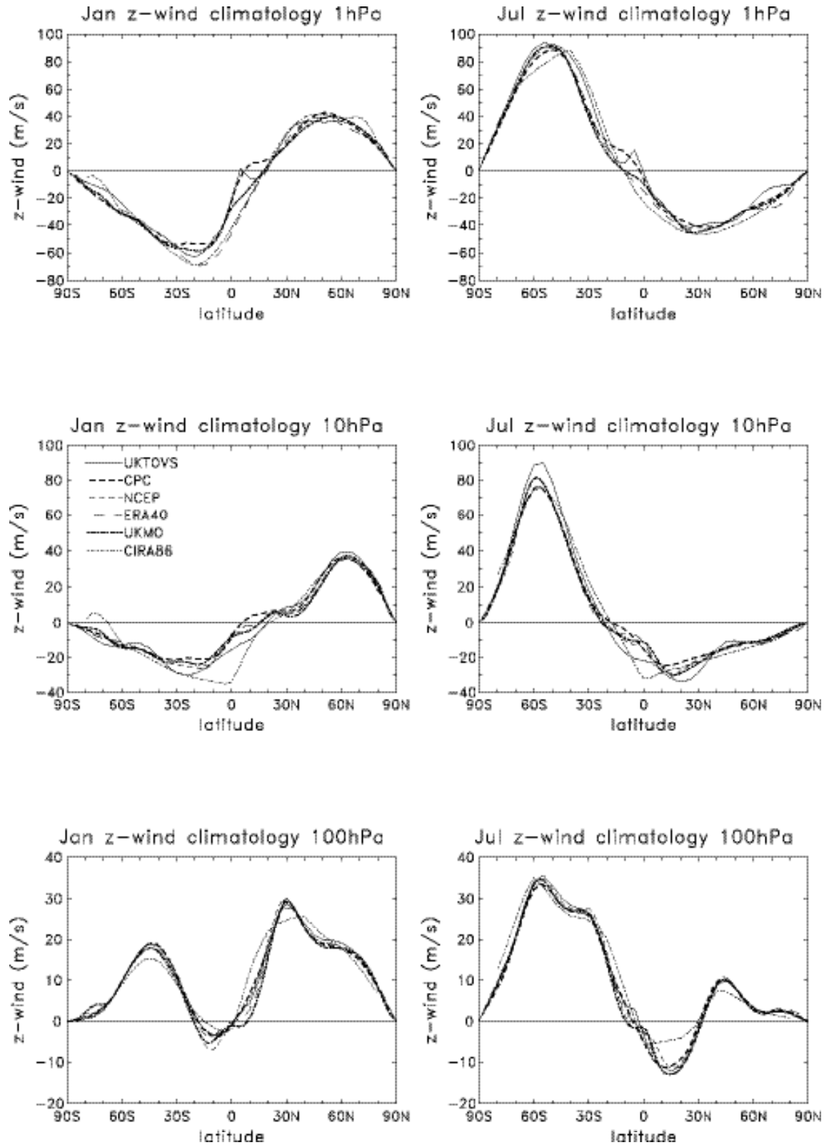
Figure 37. Latitudinal structure of zonal mean zonal wind from various analyses for January (left) and July (right), for statistics at 1 hPa (top), 10 hPa (middle) and 100 hPa (bottom).
