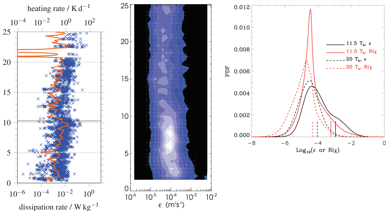
Figure 6: (left) Heating rate (in ^{\circ}K/day ) and turbulent energy dissipation rate, \epsilon in W/kg for the BEXUS 8 flight computed by spectral fitting as in Schneider et al. (2015), as a function of altitude (in km). (middle) Turbulent dissipation rate, \epsilon derived from Thorpe analysis of Riverton, WY, radiosonde data for the winter of 2007 (from Love and Geller, 2012). (right) Turbulent energy dissipation rate computed directly from DNS results in Fritts et al. (2016) over their computational domain (black curves) for two different times during the simulation 11.5 T_b and 20 T_b , where T_b is the buoyancy oscillation period for the computational basic state.
