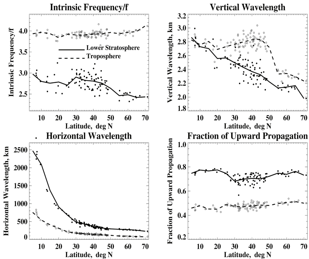
Figure 4: Five-year (1998-2002), averaged (top left) dominant intrinsic gravity wave frequency divided by the Coriolis frequency, (top right) dominant gravity wave vertical wavelength, (bottom left) dominant horizontal wavelength, and (bottom right) fractions of upward propagations as a function of latitude in the troposphere (open dots) and lower stratosphere (filled dots). The dashed and solid lines are the latitudinally binned results (with a bin size of 5°) for the troposphere and lower stratosphere, respectively. From Wang et al. (2005).
