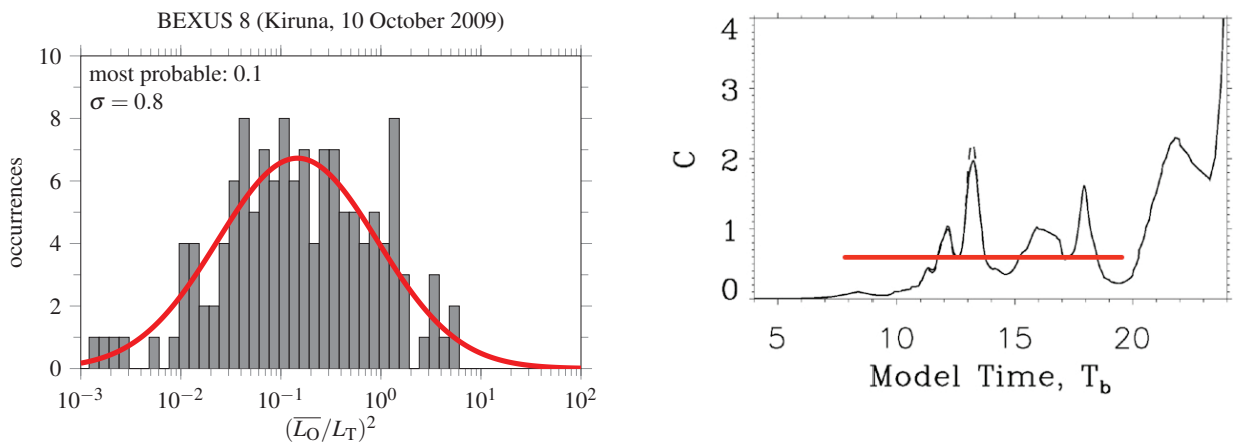
Figure 5: (left) Statistics for the ratio (L_O/L_T)^2 for LITOS measurements on the BEXUS 8 balloon flight (from Schneider et al., 2015), where the red curve is a best-fit log-normal curve. (right) Estimates for C = LO/LT from 4 to 24 T_b , where T_b is the undisturbed buoyancy oscillation period, for the full model computational domain using mean N^2 , \epsilon , L_O , and L_T for the DNS (Direct Numerical Simulation) results of Fritts et al. (2016), where the red line indicates approximately the conditions a rising balloon would be expected to encounter in determinations of L_T
