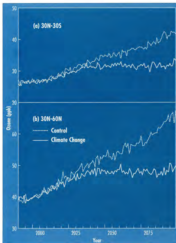
Figure 5. Abundances of ozone calculated for equatorial region (panel a) and extratropics (panel b) from the STOCHEM model where the climate is assumed to be invariant with time (control run, dashed line) and where climate changes are included (solid line). These differences arise primarily because of changes in \text{HO}_x abundances between the control runs calculations where climate changes with time. [From Johnson et al.]
