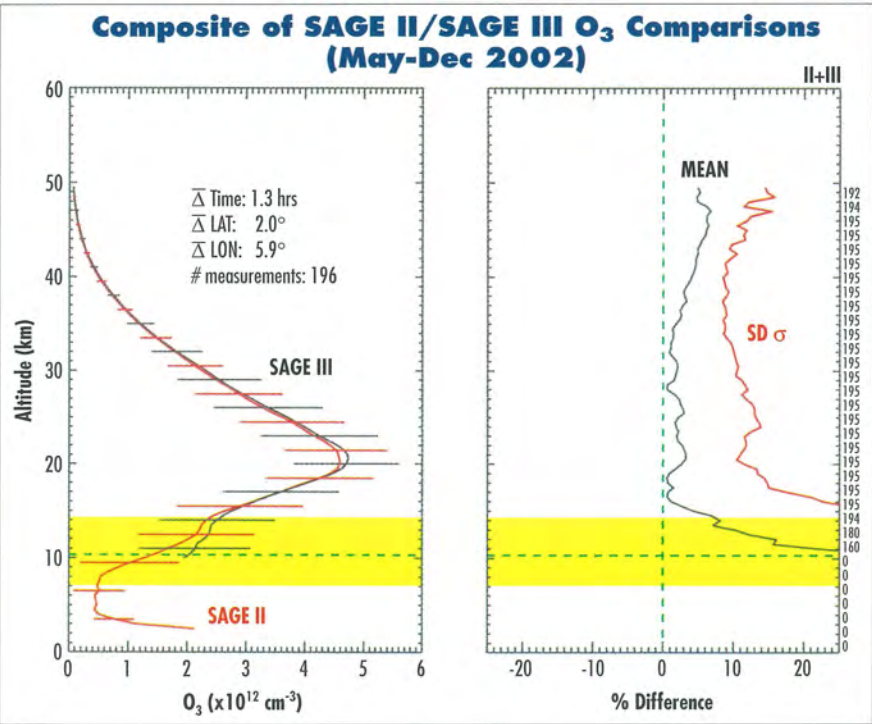
◀ Figure 1 The mean difference and standard deviation of composite comparisons between coincident SAGE III and SAGE II ozone profiles during the time period of May to December 2002 are shown. Coincidence is defined as measurements made within 4° latitude, 12° longitude, and 12 hours. For these coincidences, the mean time difference is 1.3 hours, mean latitude difference is 2°, and the mean longitude difference is 5.9°. The number of coincidences at a given altitude is given on the right hand side of the right panel. The mean is defined as SAGE III-SAGE II / the average of SAGE III + SAGE II. The yellow shading in each panel indicates the range of tropopause heights for the comparisons and the horizontal dashed green line is the mean tropopause level. Note that the two instruments agree within 3% from 15 to 40 km.
