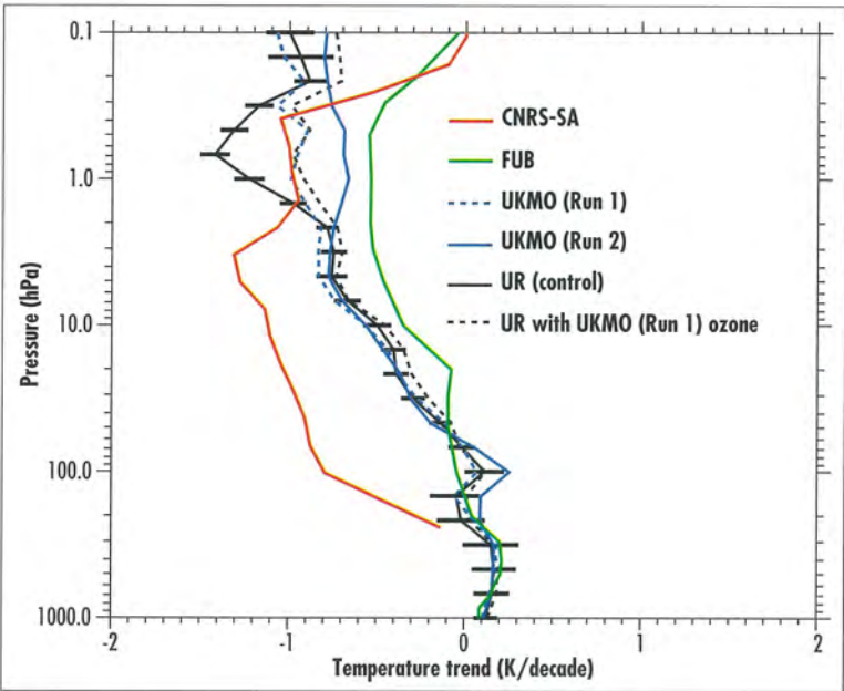
Figure 7 Simulated globally and annually averaged temperature trends in the models for the period 2000-2019 as a function of pressure. The UR results are shown as a control run with fixed ozone (black line) and a run (black broken line) with ozone from Run 1 of the UKMO simulation. The error bars in the control run indicate the 95 % confidence intervals. For clarity, the uncertainties are not included in the other model simulations but are of similar magnitude.
