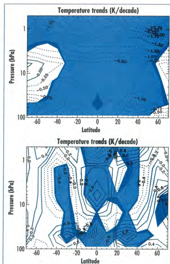
Figure 3. Top panel: Annually averaged temperature trend from the SSU/MSU data. The light and dark shading indicates where the trend is significantly different from zero at the 90 % and 95 % levels, respectively. Bottom panel: The QBO component of the temperature signal observed by SSU/MSU instruments. The units are K per QBO cycle assuming a 7 month phase lag. The statistical significance of the signal is indicated for the 90 % and 95 % as light and dark blue, respectively.
