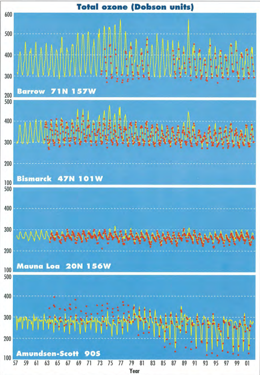
◀ Figure 1 Timeseries of monthly mean total ozone in DU from independent ground based observations (red dots) and ERA-40 (yellow curve) for the stations Barrow, Bismarck, Mauna Loa, and Amundsen-Scott. [Figure provided by A. Simmons, following similar calculations by P. Simon].
