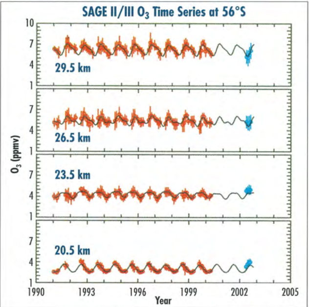
► Figure 4 Time-series of SAGE II (red circles) and SAGE III (blue circles) monthly zonal averages centered near 56°S is plotted for a number of altitudes. The black line is the model fit of SAGE II ozone data between October 1984 and June 2000, and extended to August 2002. It is clear that the SAGE III data follow the natural seasonal cycle (climatology) and «fill in» monthly gaps of the SAGE II time series. The SAGE II model climatology consists of a mean, linear trend, seasonal, quasi-biennial oscillation, and Solar cycle terms.
