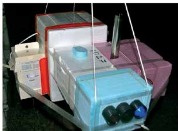
Figure 8: Left: Locations and number of sondes launched for the first six years of the SWOP project (LS: Lhasa, KM: Kunming). Right: Image of the integrated four-sensor payload with ECC, RS, CFH/FPH, and COBALD.
