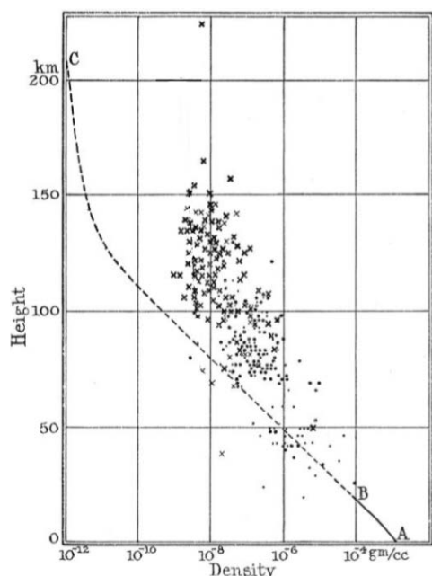
Figure 11: The density of the atmosphere as a function of height determined from observations of the appearance and disappearance of visible meteor trails. Each cross (dot) shows a determination for an individual meteor of the density at appearance (disappearance). The larger (smaller) crosses and dots show results from trails seen by multiple (single) skilled observers. The dashed curve shows the density expected if the temperature everywhere above 20 km was 220 K. Figure adapted from Lindemann and Dobson (1923).
