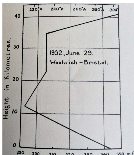
Figure 12: Inferred temperature as a function of height based on observations made on June 29, 1932, of acoustic propagation between a source at Woolwich and an array of microphones at Bristol about 180 km away. From Whipple (1934).
