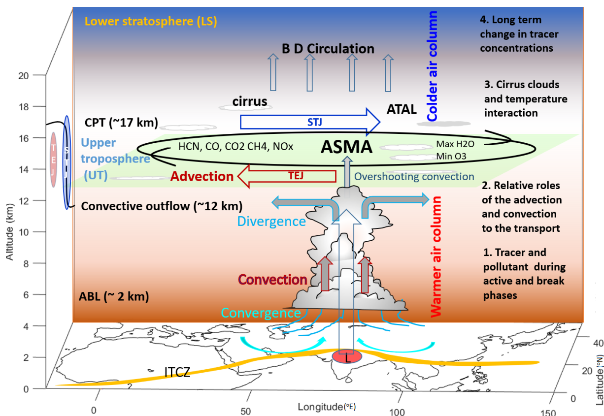
Figure 8: Schematics of the vertical structure of the troposphere (red) and lower stratosphere (blue) showing the transport of the surface pollutant over the Indian monsoon region. The Asian summer monsoon anticyclone (ASMA, green) horizontally confined within subtropical jet (STJ) in the northern flank and tropical easterly jet (TEJ) in equatorial side and vertically confine within top of the convective outflow level and cold point tropopause (CPT). During ASM inter tropical convergence zone (ITCZ) shifts towards the northward create low pressure in central India. The deep convection transports the surface pollutants from the South Asian atmospheric boundary layer (ABL). ASMA contains chemically active gases and surface pollutants which is slowly enters to the deep stratosphere possibly by Brewer-Dobson circulation. Four main subthemes of the conference are listed in the diagram.
