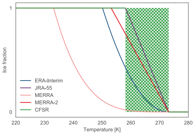
Figure 2.3: Partitioning of cloud condensate into liquid and ice in five recent reanalyses.
