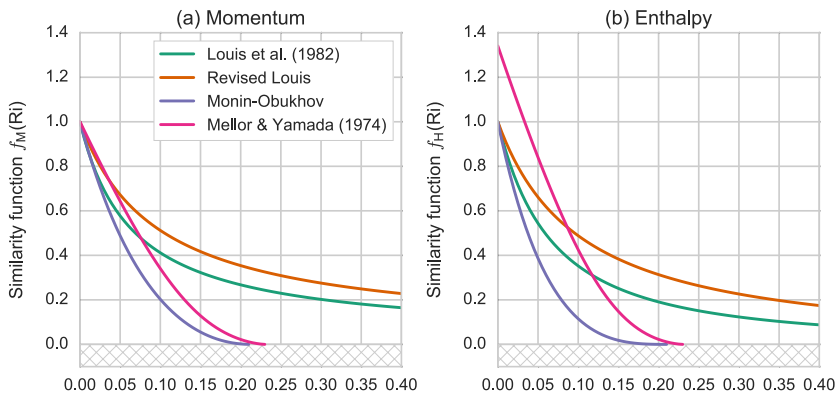
Figure 2.4: Similarity functions for selected turbulence schemes implemented in recent reanalysis systems.
