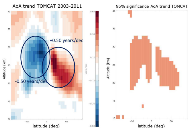
Figure 5.38: Cross-section of the linear trend (years per decade) of the mean AoA for the period 2003–2011 from the TOMCAT simulation with ERA-Interim (left); red colours indicate positive trends and blue colours negative trends. Regions where the trend is significant at least to the 95% confidence level are shown by the shaded areas in the right panel. The dipole structure in the mean AoA displays maximum positive values over the NH middle stratosphere midlatitudes of up to 0.50 years/decade, and minimum values of up to -0.50 years/decade. (From Monge-Sanz et al., in prep).
