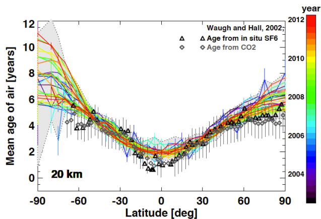
Figure 5.23: Comparison of MIPAS-derived AoA (coloured lines) as a function of latitude at 20 km of altitude with airborne AoA measurements on basis of SF 6 (triangles) and CO 2 (diamonds). Shown for MIPAS is the monthly zonal mean for every third month between July 2002 and March 2012. The grey shaded area is the range of variability of all MIPAS zonal mean data. The vertical error bars are measurement uncertainties for CO 2 -derived airborne AoA measurements. Airborne measurements are shown after Waugh and Hall (2002) and Hall et al. (1999). Figure from Haenel et al. (2015, Supplement).
