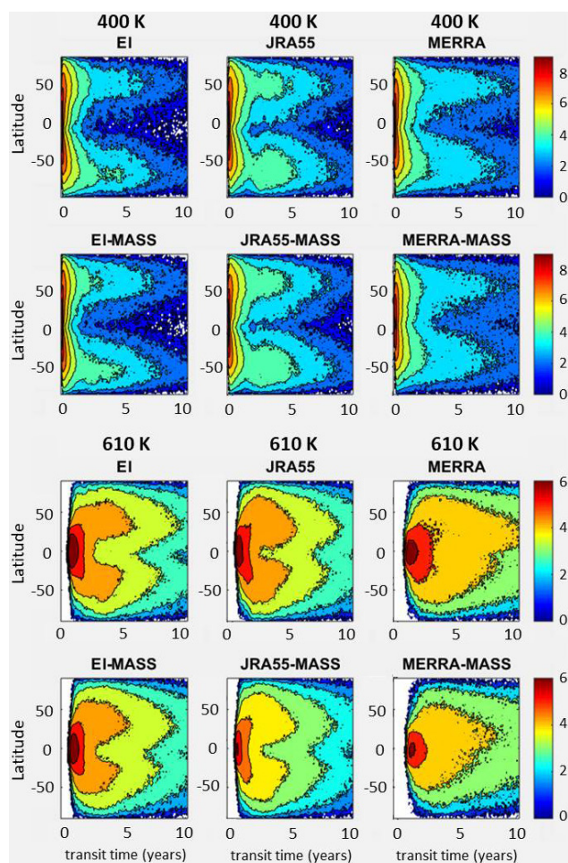
Figure 5.35: Horizontal sections of the age spectrum as a function of latitude for two different levels: 400 K (top), and 610 K (bottom), as obtained from TRACZILLA simulations with ERA-Interim (left), JRA-55 (centre) and MERRA (right), without mass correction (upper row) and with mass correction (lower row).
