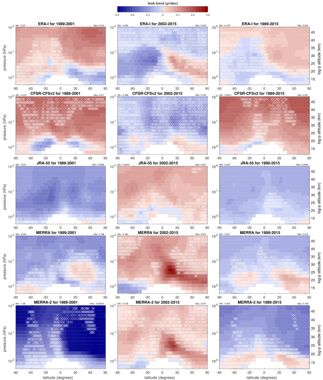
Figure 5.39: Latitude-pressure distributions of AoA trends (years/decade) over 1989–2001 (left column), 2002–2015 (middle column) and 1989–2015 (right column) using the five reanalyses (from top to bottom: ERA-I, CFSR, JRA-55, MERRA, MERRA-2). White crosses indicate where the sign of the trend is not significant at the 95% confidence level. Darker blues indicate more negative trends and darker reds more positive trends. Figure from Chabrilat et al. (2018) .
