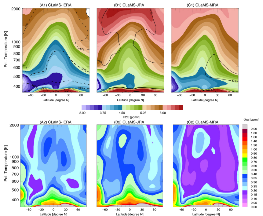
Figure 5.47: The zonal and annual mean of water vapor (ppmv) from reanalysis-driven CLaMS simulations, averaged over the period 1980–2013 (top panel). In the bottom panel, the total variances (relative to the climatology) of respective monthly means are shown. The black contours show the differences of each CLaMS run relative to the means of (A1), (B1) and (C1). The reanalyses used are ERA-Interim (left), JRA-55 (middle) and MERRA-2 (right).
