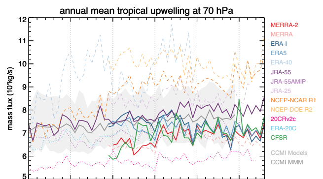
Figure 5.13: Time series of annual mean tropical upwelling mass flux at 70 hPa (between turnaround latitudes). Line styles as Figure 5.4 . The gray shading denotes the range of CCM models with the multi-model mean shown as thick gray line.
