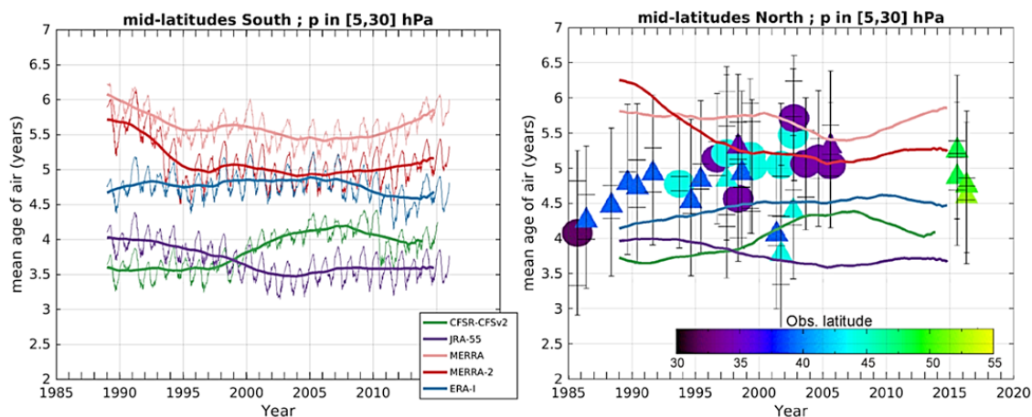
Figure 5.36: Time evolution of AoA averaged from 30 hPa to 5 hPa (approximately 24 km to 36 km) in the southern ( 50^{\circ}\text{S} – 40^{\circ}\text{S} , left) and northern mid-latitudes ( 40^{\circ}\text{N} – 50^{\circ}\text{N} , right). Solid lines show model output with color codes according to the legend shown in the left panel. Thin lines (left panel only; omitted from right panel for clarity) show instantaneous model output every 5 days while thick lines are smoothed with a one-year running mean. Northern mid-latitude symbols (right panel) represent values derived from balloon observations of \text{SF}_6 (circles) and \text{CO}_2 (triangles) with color code showing the latitude of the measurements and outer error bars including sampling uncertainties (Engel et al., 2017). Adapted from Chabrillat et al. (2018).
