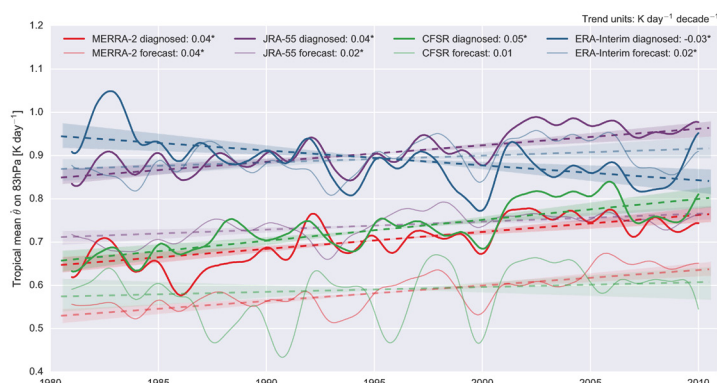
Figure 5.20: Time series of the tropical mean ( 30^{\circ}\text{S} - 30^{\circ}\text{N} ) of the diabatic heating rate field ( \text{K/day} ) at the 83 hPa level for the diagnosed field (darker solid lines) and for the forecast field (lighter solid lines). The corresponding linear trends ( \text{K/day-decade} ) are also shown (dashed lines). Time series have been low-pass filtered via a 24-month rolling mean using a Hamming window. Trends are calculated from annual mean values via the Theil-Sen estimator (95 % confidence intervals estimated via bootstrapping). The best-estimate trend values are shown in the legend. Reanalyses shown and colour scale as in Figure 5.19 .
