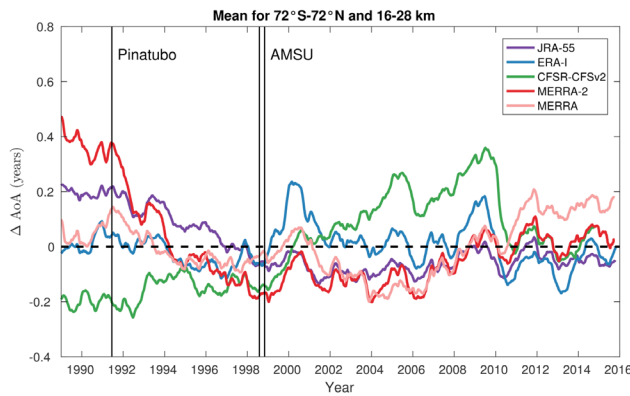
Figure 5.45: Time evolution of the globally averaged ( 72^{\circ}\text{S} - 72^{\circ}\text{N} ) anomalies of AoA with respect to their mean (1989 - 2015) annual cycles, between 16 km and 28 km, using the five reanalyses with same colour codes as in Figure 5.36 . The black vertical lines highlight the start of the Pinatubo eruption and the first assimilation of AMSU data. From Chabrillat et al. (2018).
