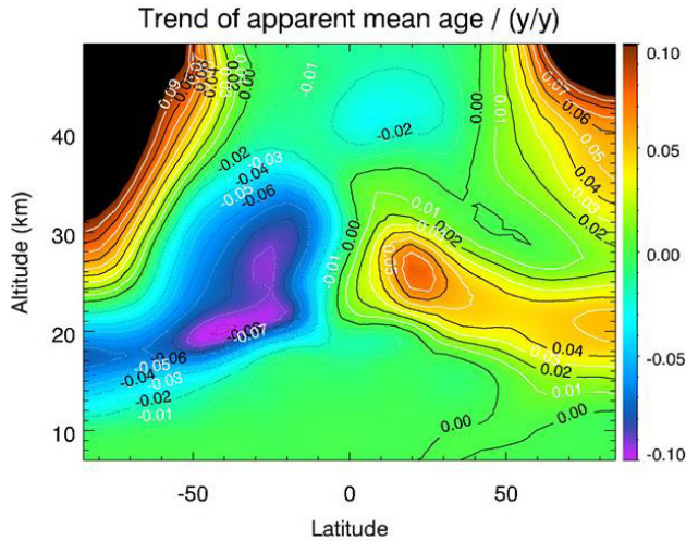
Figure 5.41: Trend of the apparent mean AoA (expressed as the lag time) of the \text{SF}_6 tracer T3 in the KASIMA simulation with ERA-Interim (2002 - 2012), when including mesospheric loss for \text{SF}_6 .
