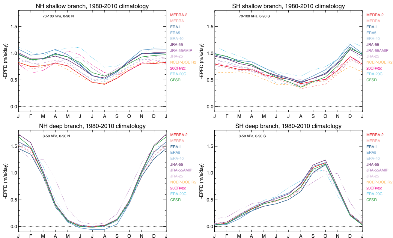
Figure 5.4: Climatological (1980 - 2010) seasonal evolutions for each reanalysis of the EP-flux divergence for the shallow and deep BDC branches and for each hemisphere separately. Full lines refer to more recent reanalysis products, dashed lines to older reanalysis products, and dotted lines to other products.
