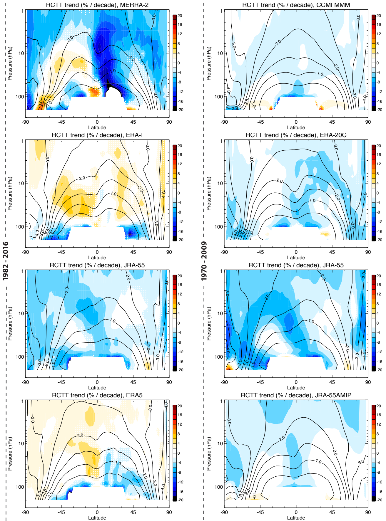
Figure 5.17: Trends in annual mean RCTT as a function of latitude and pressure (color shading, in %/decade) for the period 1982-2016 in the recent reanalysis products (left column, note that ERA5 is included instead of CFSR, see text), as well as the period 1970-2009 in the products shown (right column). Each product's climatology over the respective period is depicted as black contours.
