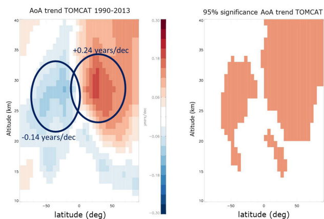
Figure 5.37: Cross-section of the linear trend (years per decade) of the mean AoA for the period 1990–2013 from the TOMCAT simulation with ERA-Interim fields (left); red colours indicate positive trends and blue colours negative trends. Regions where the trend is significant at least to the 95% confidence level are shown by the shaded areas in the right panel. The dipole structure in the mean AoA displays maximum positive values over the NH middle stratosphere midlatitudes of up to 0.24 years/decade, and minimum values of up to -0.14 years/decade. Updated from Monge-Sanz et al. (2012).
