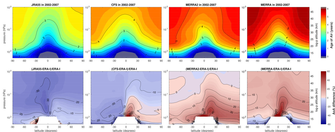
Figure 5.28: Latitude-pressure distribution of mean AoA averaged over the period 2002–2007 from BASCOE simulations driven by all reanalyses but ERA-Interim (top row). The reanalyses are, from left to right, JRA-55, CFSR, MERRA-2 and MERRA. The bottom row shows corresponding relative differences with respect to the mean AoA from the ERA-Interim-driven simulation in Figure 5.26 ; darker blue indicates more negative differences and darker red more positive differences. Figure from Chabrilat et al. (2018).
