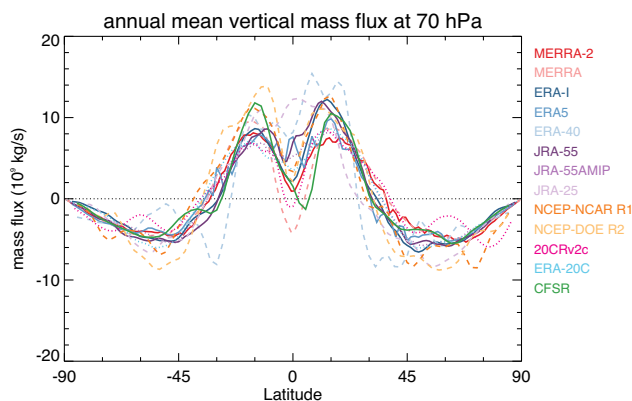
Figure 5.5: Climatological (1980 - 2010) vertical mass flux at 70 hPa as a function of latitude for the annual mean. Line styles as in Figure 5.4.
