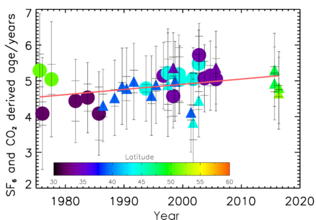
Figure 5.22: Time series of mean age derived from balloon observations. Data before 2010 are from Engel et al. (2009), while data from 2015 and 2016 are derived from the AirCore measurements in Engel et al. (2017). Each data point represents the average mean AoA between 5–30 hPa. Error bars represent the variability (inner error bars), and the uncertainty (outer error bars) as discussed in Engel et al. (2009). A non-significant trend of 0.15 (\pm 0.18) years per decade is derived from these observations. Figure from Engel et al. (2017).
