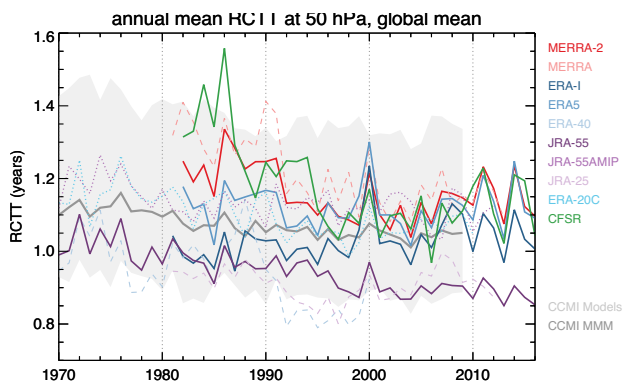
Figure 5.16: Time series of annual global mean RCTTs at 50 hPa. Line styles as Figure 5.4 . The gray shading denotes the range of CCMi models with the multi-model mean shown as thick gray line.
