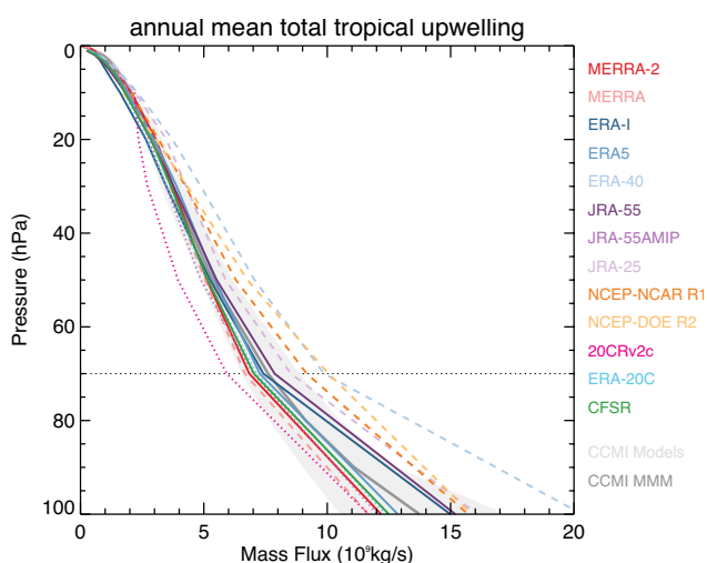
Figure 5.8: Climatological annual mean total tropical upwelling as a function of pressure (between turnaround latitudes at each level). Line styles as Figure 5.4 . Gray shading shows range of CCMi models with the thick gray line marking the MMM.
