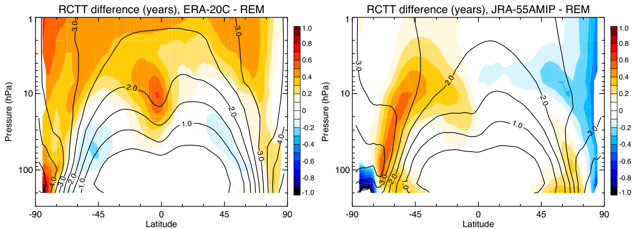
Figure 5.12: As Figure 5.11 but for ERA-20C (left, end year is 2010) and JRA-55AMIP (right, end year is 2012).
