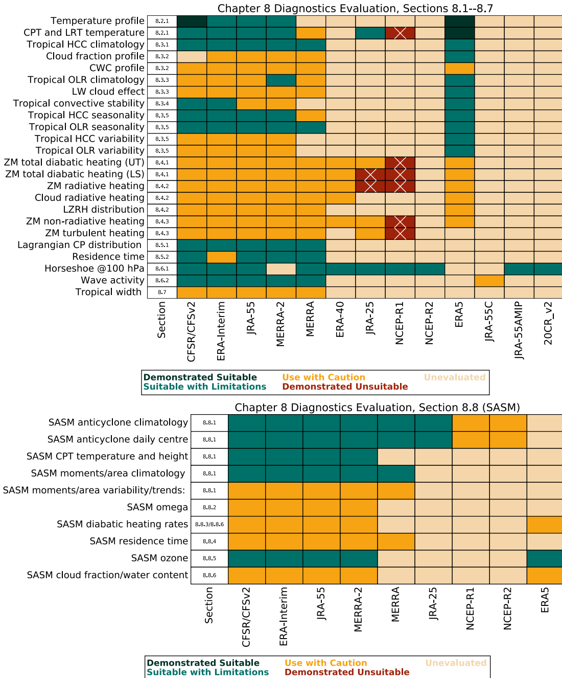
Figure 8.72: Diagnostic evaluation for Chapter 8 on the Tropical Tropopause Layer (TTL). Top: Climatological and dynamical TTL characteristics (Sections 8.2-8.7) and bottom: South Asian Summer Monsoon (SASM) characteristics (Section 8.8). CPT: Cold Point Tropopause, LRT: Lapse Rate Tropopause, HCC: High Cloud Cover, CWC: Cloud Water Content, OLR: Outgoing Longwave Radiation, LW: Long Wave, ZM: Zonal Mean, UT: Upper Troposphere, LS: Lower Stratosphere, LZRH: Level of Zero Radiative Heating, CP: Cold Point.
