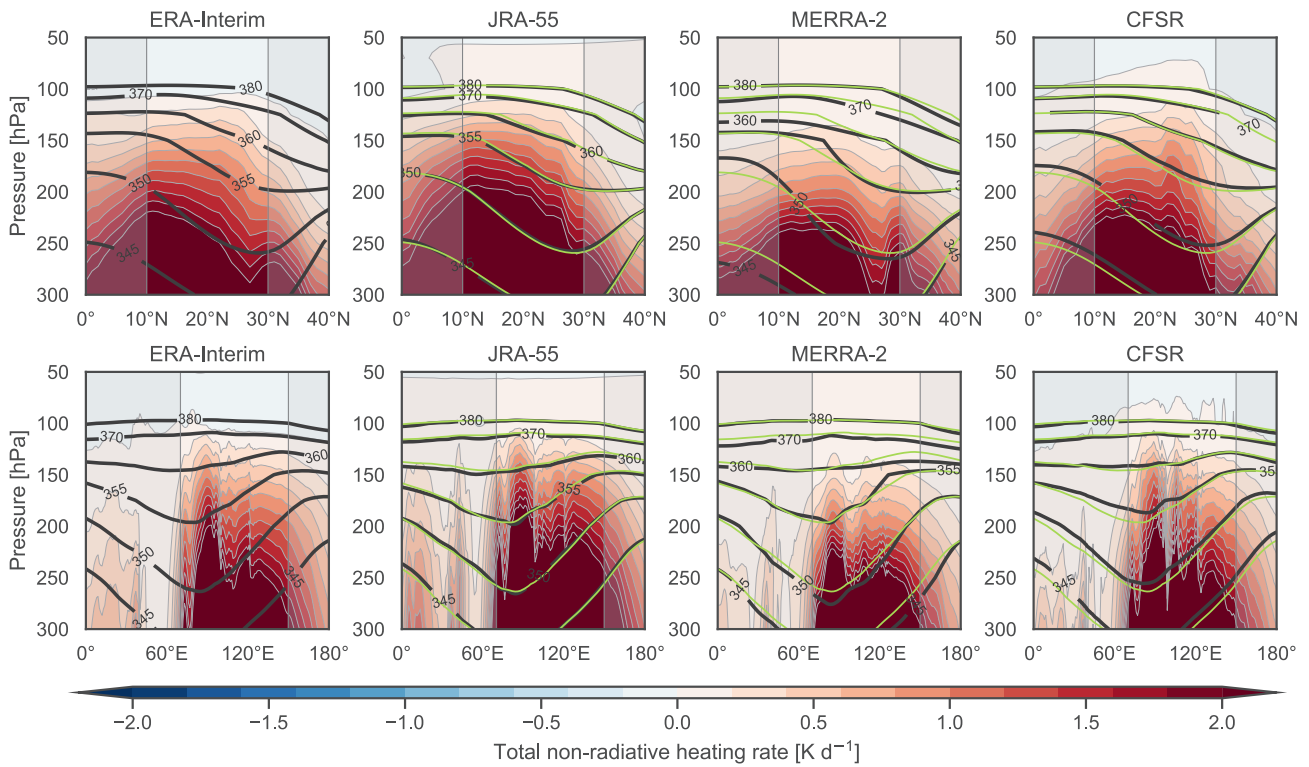
Figure A8.9: As in Fig. 8.59, but for non-radiative heating [ K day^{-1} ] averaged over JJA 1980-2010. Zonal means are calculated over 70^{\circ} - 150^{\circ}E (vertical lines in lower panels); area-weighted meridional means over 10^{\circ} - 30^{\circ}N (vertical lines in upper panels). ERA-Interim potential temperature contours are shown in light green on the JRA-55, MERRA-2, and CFSR panels for ease of comparison.
