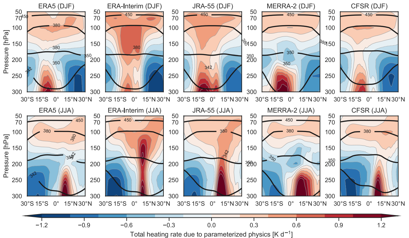
Figure A8.4: As in Fig. 8.20, but for zonal mean total diabatic temperature tendencies ( Q/c_p in K day^{-1} ; shading and gray contours) and potential temperature ( \theta in K; black contours) averaged over 1980–2010 for the solstice seasons DJF (upper row) and JJA (lower row).
