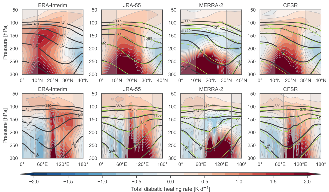
Figure 8.59: Zonal and meridional mean total diabatic heating rates due to parameterized physics ( K day^{-1} , shading) and potential temperature (K, contours) during JJA 1980-2010 within the SASM region. Zonal means are calculated over 70-150^{\circ}E (vertical lines in lower panels); area-weighted meridional means over 10-30^{\circ}N (vertical lines in upper panels). ERA-Interim potential temperature contours are shown in light green on the JRA-55, MERRA-2, and CFSR panels for ease of comparison.
