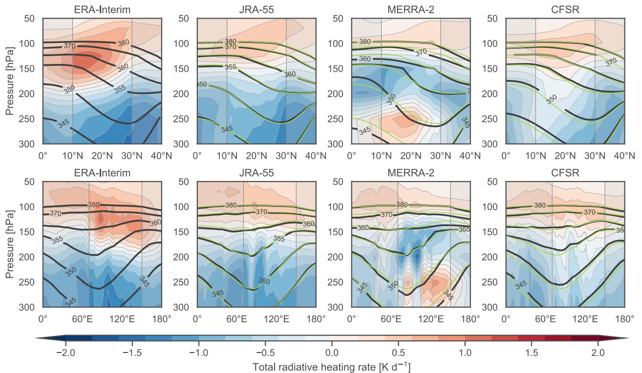
Figure A8.7: As in Fig. 8.59 but for all-sky radiative heating [ K day^{-1} ] averaged over JJA 1980–2010. Zonal means are calculated over 70^{\circ} - 150^{\circ} E (vertical lines in lower panels); area-weighted meridional means over 10^{\circ} - 30^{\circ} N (vertical lines in upper panels). ERA-Interim potential temperature contours are shown in light green on the JRA-55, MERRA-2, and CFSR panels for ease of comparison.
