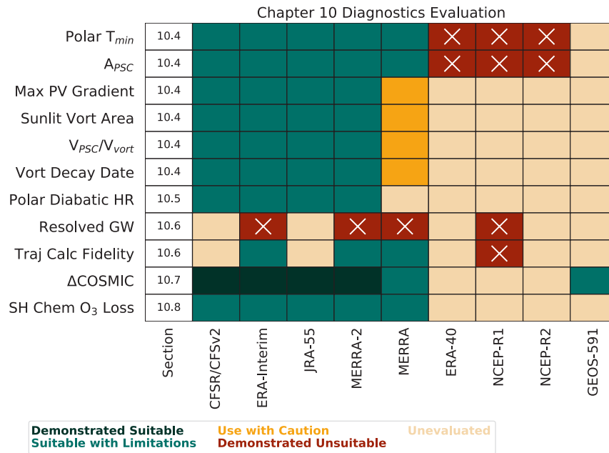
Figure 12.10: (Same as Figure 10.26.) A summary of the diagnostics evaluated in Chapter 10: Polar Processes. The “Section” column at left indicates where in the chapter each diagnostic is described. See the beginning of this chapter for the meaning of the evaluation terms. “Polar T_{min} ” = minimum temperatures poleward of 40°S; “ A_{PSC} ” = area of temperatures below PSC existence thresholds; “Max PV Gradient” = daily maximum gradients in potential vorticity, a measure of vortex strength; “Sunlit Vort Area” = area of the polar vortex in sunlight; “ V_{PSC}/V_{vort} ” = winter-mean volume of air with temperature below the nitric acid trihydrate PSC threshold, expressed as a fraction of the volume of air in the vortex; “Vort Decay Date” = the last day before which the vortex area is above 1 % of a hemisphere continuously for 30 days; “Polar Diabatic HR” = Diabatic heating rates in the polar vortex region; “Resolved GW” = resolved atmospheric gravity wave spectrum; “Traj Calc Fidelity” = fidelity of reanalysis-driven trajectory calculations from a Lagrangian transport model; “ \Delta COSMIC” = differences between reanalysis and COSMIC GNSS-RO temperatures; “SH Chem O 3 Loss” = estimates of chemical loss in the Antarctic ozone hole from a chemistry transport model forced by reanalyses.
