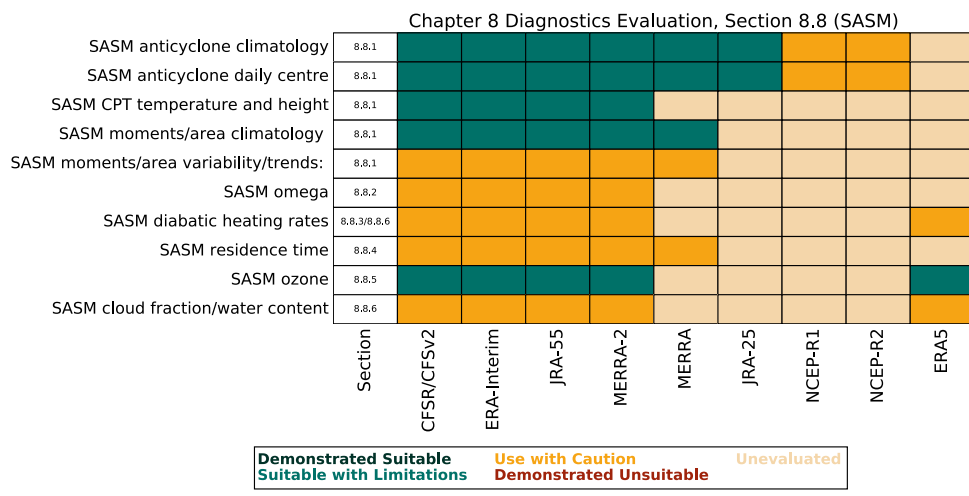
Figure 12.8: (Same as Figure 8.72, bottom.) A summary of the diagnostics evaluated in Section 8.8 of Chapter 8: South Asian Summer Monsoon (SASM). The "Section" column at left indicates where in Section 8.8 each diagnostic is described. See the beginning of this chapter for the meaning of the evaluation terms. "CPT" = cold point tropopause.
