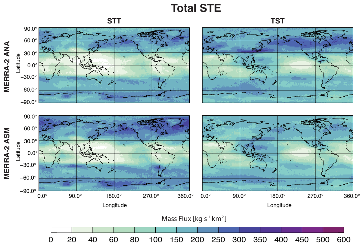
Figure 7.18: A comparison of (top) MERRA-2 ANA panels from Figure 4 of Boothe and Homeyer (2017) and (bottom) the revised MERRA-2 ASM analysis. Global distributions of annual-mean (left) STT and (right) TST. These STE estimates were calculated using a trajectory model.
