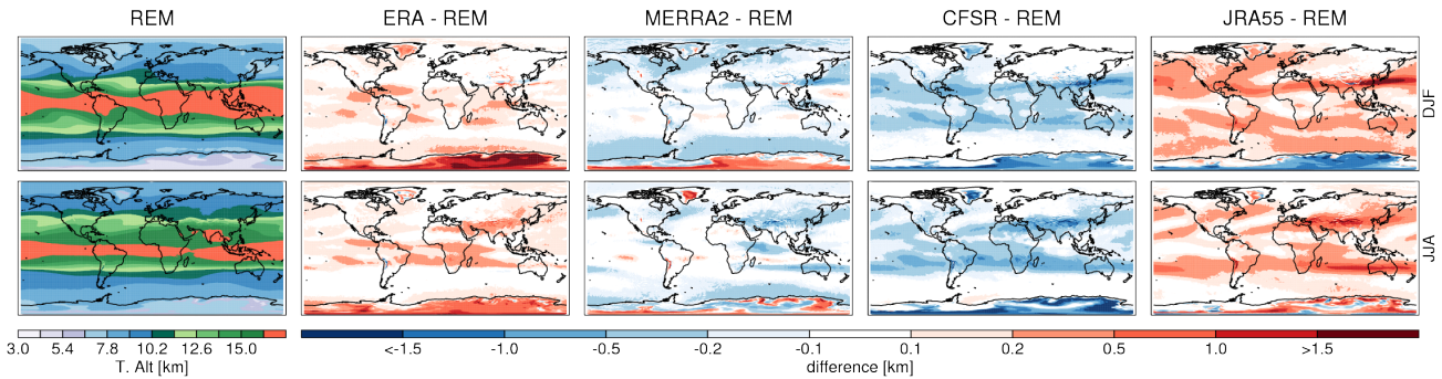
Figure 7.4: Climatological (1980 - 2014) 2 PVU tropopause altitudes for DJF (top row) and JJA (bottom), from the REM for the four reanalyses, and (second through rightmost panels) the difference of each reanalysis from the REM (reanalysis – REM) for that climatological period. Adapted from Millán et al. 2021.
