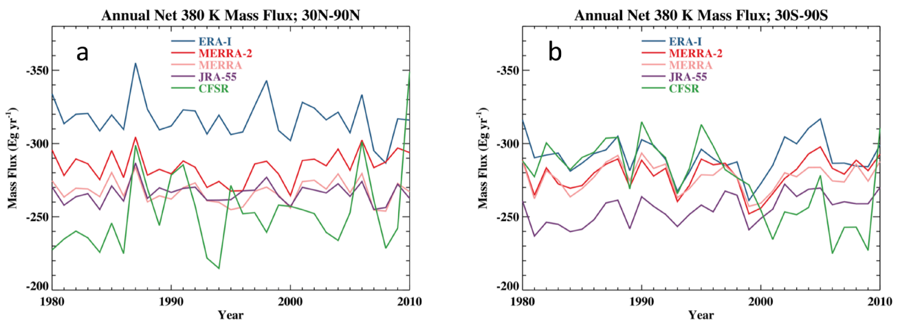
Figure 7.24: Time series for 1980 through 2010 of the annual net mass flux integrated from 30°–90° latitude in (a) the NH and (b) the SH. Values are in 10 18 g yr -1 and negative values denote a net downward flux.
