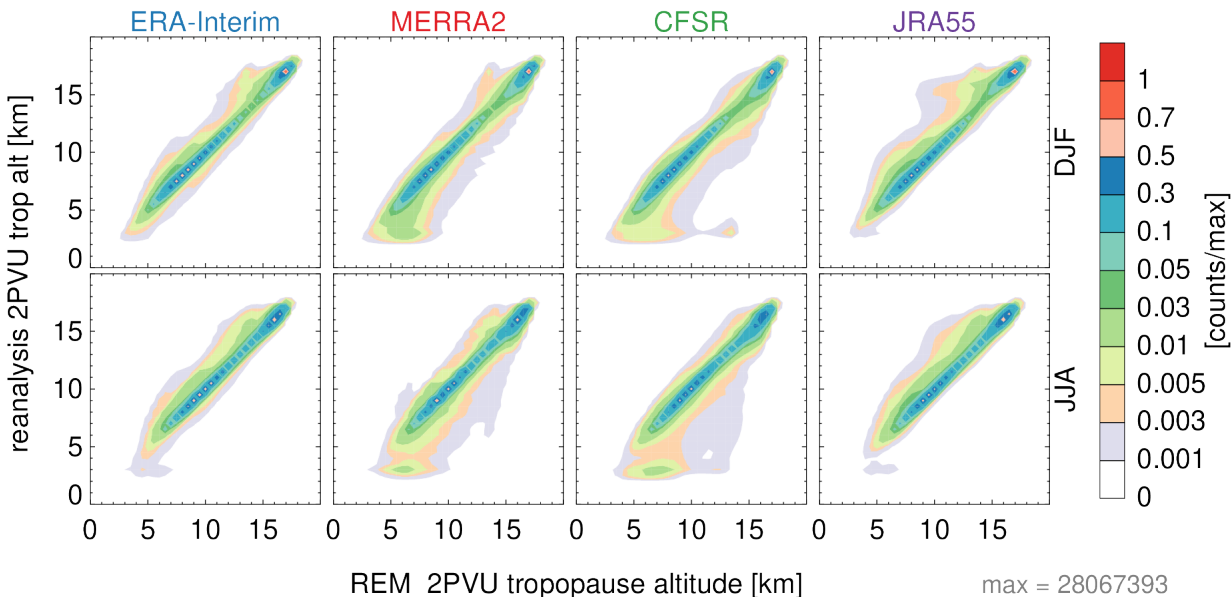
Figure 7.5: Density plots of REM tropopause altitude (x-axis) versus tropopause altitude for each of four reanalyses (y-axis), for DJF (top) and JJA (bottom), for 1980 - 2014. Adapted from Millán et al. 2021.
