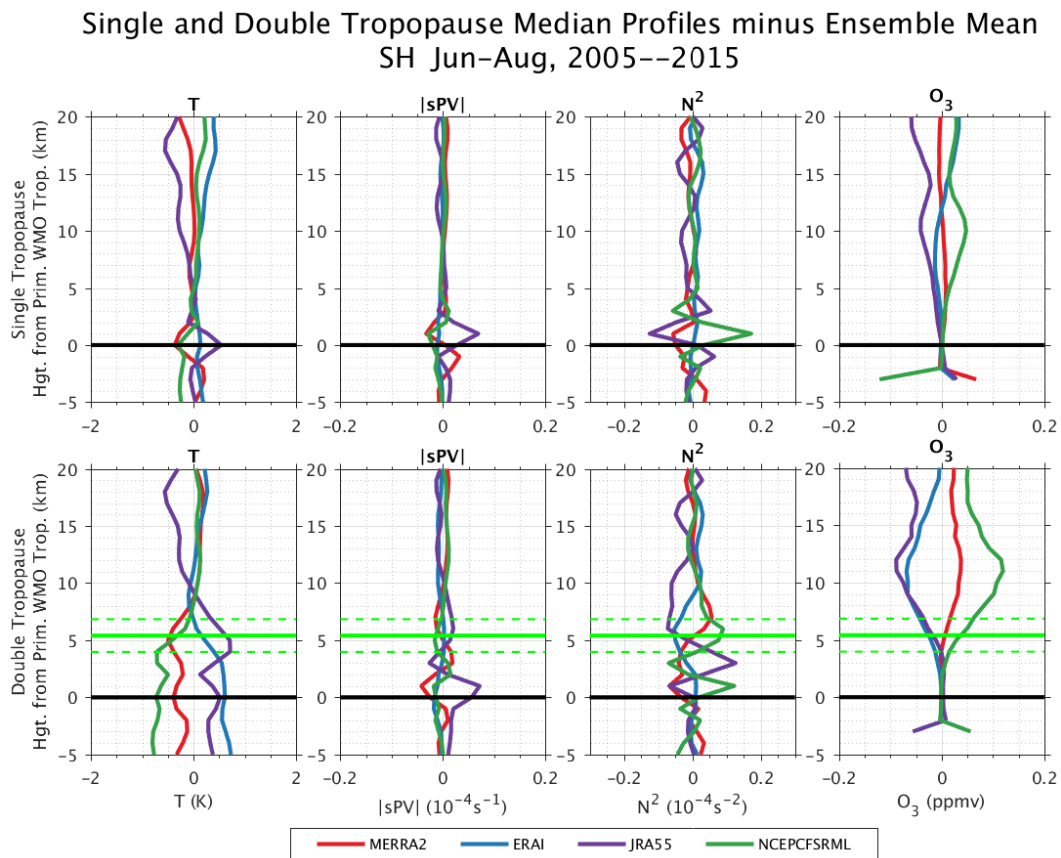
Figure 7.9: As in Figure 7.8 but for the SH in JJA.
