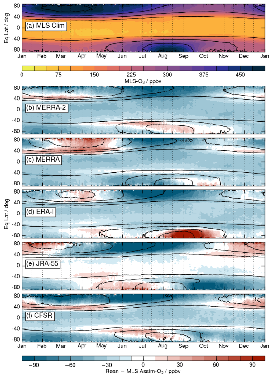
Figure 7.28: Climatological (2005–2015) annual cycle of ozone as a function of EqL at 340 K, showing (top) v4.2 MLS ozone and (following rows) difference (reanalysis – MLS) of MLS from each of the MERRA-2, MERRA, ERA-Interim, JRA-55, and CFSR/CFSv2 reanalyses. The black overlays show the same selected ozone contours, from MLS on the top panel and each of the reanalyses on the following panels.
