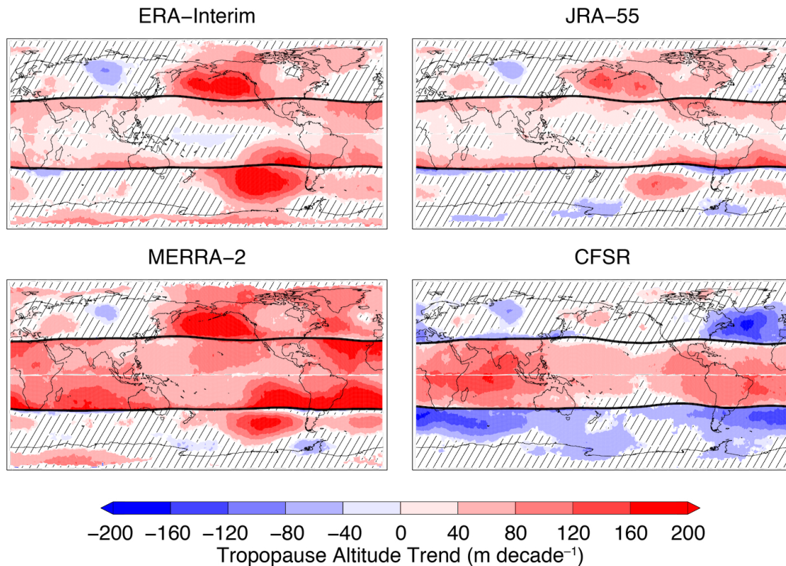
Figure 7.3: Maps of 35-yr (1981 - 2015) trends in the WMO lapse-rate tropopause altitude in a tropopause break-relative latitude coordinate from four modern reanalyses: ERA-Interim, JRA-55, MERRA-2, and CFSR/CFSv2. Color-filled regions are statistically significant at the 99% level. Thick black lines show the annual-mean tropopause break latitudes for each reanalysis. Figure 5 from Xian and Homeyer (2019).
