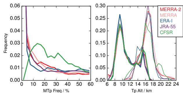
Figure 7.7: Summary of globally / seasonally averaged frequency distributions of multiple tropopause frequencies (left) and altitudes (right; primary tropopause thick lines, secondary tropopause thin lines) in five reanalyses. Adapted from Manney et al. , 2017.
