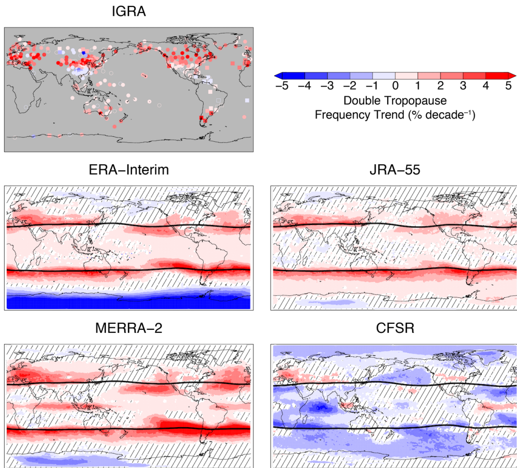
Figure 7.10: Maps of 35-yr (1981 - 2015) trends in the WMO lapse-rate tropopause double tropopause frequency from global radiosonde observations and four modern reanalyses: ERA-Interim, JRA-55, MERRA-2, and CFSR/CFSv2. Color-filled regions are statistically significant at the 99% level. Thick black lines show the annual-mean tropopause break latitudes for each reanalysis. From Xian and Homeyer (2019).
