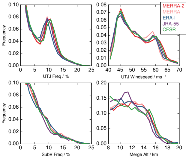
Figure 7.13: Summary of globally / seasonally averaged frequency distributions for (a) upper tropospheric jet frequency distributions and wind speeds and (b) subvortex jets in five reanalyses. Adapted from Maney et al., 2017.
