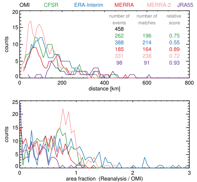
Figure 7.35: (Top) Histograms of the distance between the mini-hole events found in the reanalysis fields and the ones found in OMI data (Black, green, blue, red, pink, purple lines represent OMI, CFSR, ERA-Interim, MERRA, MERRA-2, and JRA-55 respectively). Also shown is the total number of events as well as the number of matches between the events found in OMI and in the reanalyses. (Bottom) Histograms of the area fraction of mini-hole events. (From Millan and Manney, 2017.)
