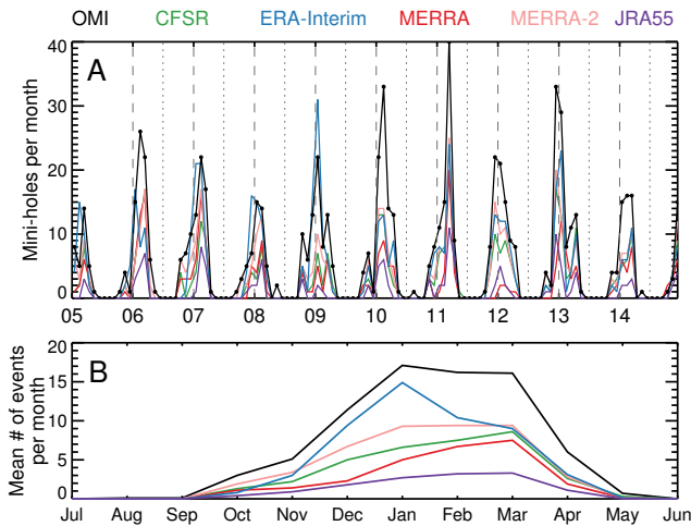
Figure 7.34: (A) Mini-hole events per month during 2005–2014 in the Northern Hemisphere as found in OMI data and reanalysis fields (black, green, blue, red, pink, purple lines represent OMI, CFSR/CFSv2, ERA-Interim, MERRA, MERRA-2, and JRA-55 respectively). Dashed vertical lines indicate the beginning of each January, dotted vertical lines the beginning of each July. (B) Mean number of mini-hole events in a given month (during 2005–2014). (From Millan and Manney, 2017.)
